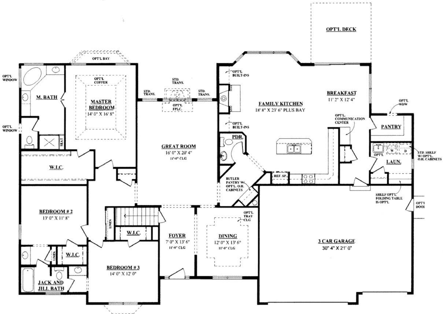
Floor Plan
